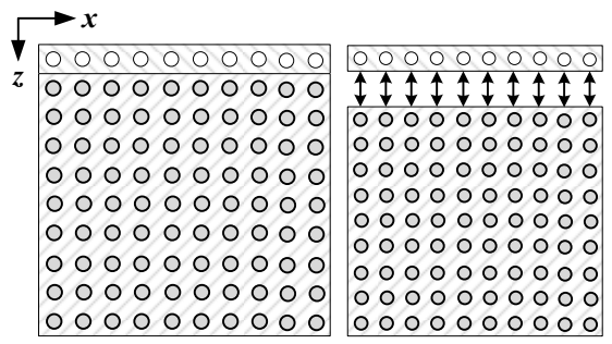
Figure 3. The grid used for the numerical solution with the conventional approach (left) and component-based approach (right)
